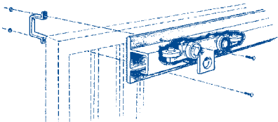
Square Frame Kit
