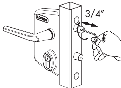
Keeper installation drawing
