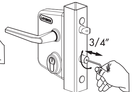
Keeper installation drawing
