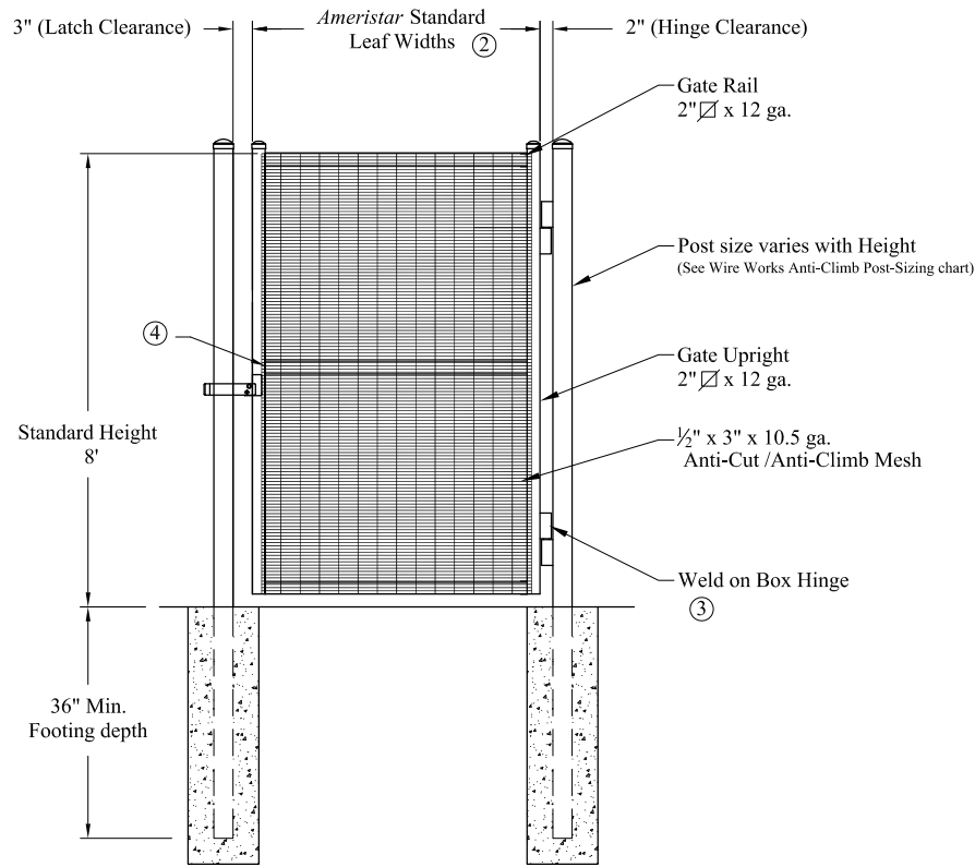
Single gate Arrangement
