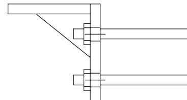
Truck Bracket
