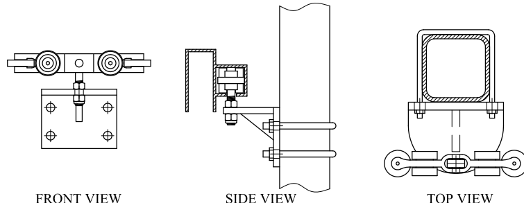
DETAIL C
