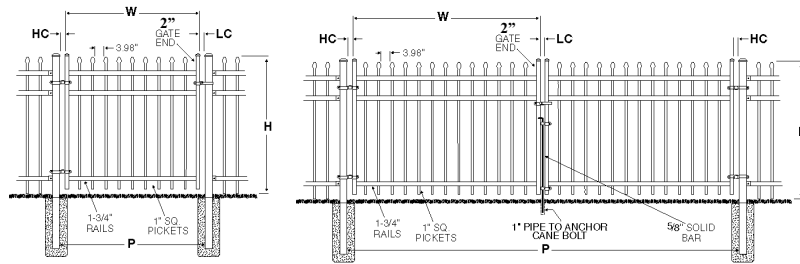
Order 1 Leaf For Single Swing Opening
