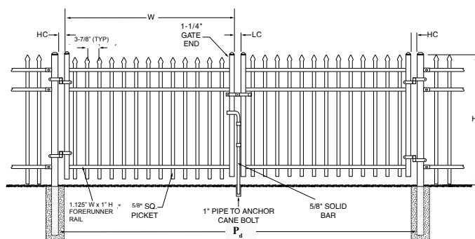
Order 2 Leaves For Double Swing Opening
