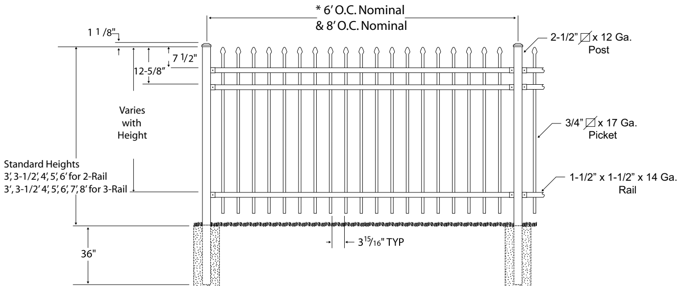
TYPICAL PANEL DRAWING (Classic Style shown; Warrior, Majestic, and Genesis also available)
