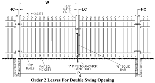
Order 2 Leaves For Double Swing Opening
