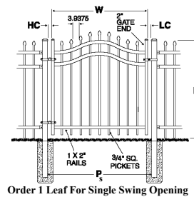
Order 1 Leaf For Single Swing Opening (Available only as single)
