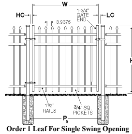
Order 1 Leaf For Single Swing Opening
