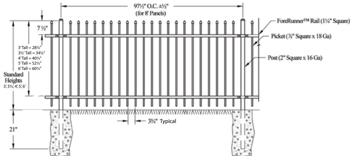
TYPICAL PANEL DRAWING (Classic Style shown; Warrior, Majestic and Genesis also available)
