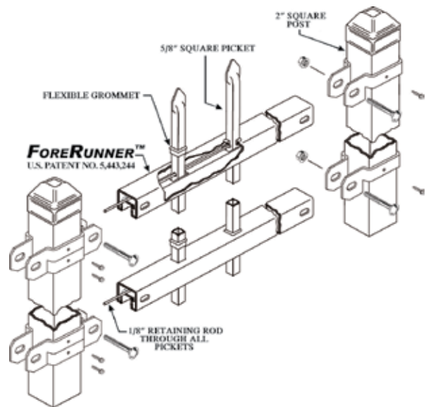
TYPICAL PANEL DRAWING (Classic Style shown; Warrior, Majestic and Genesis also available)
