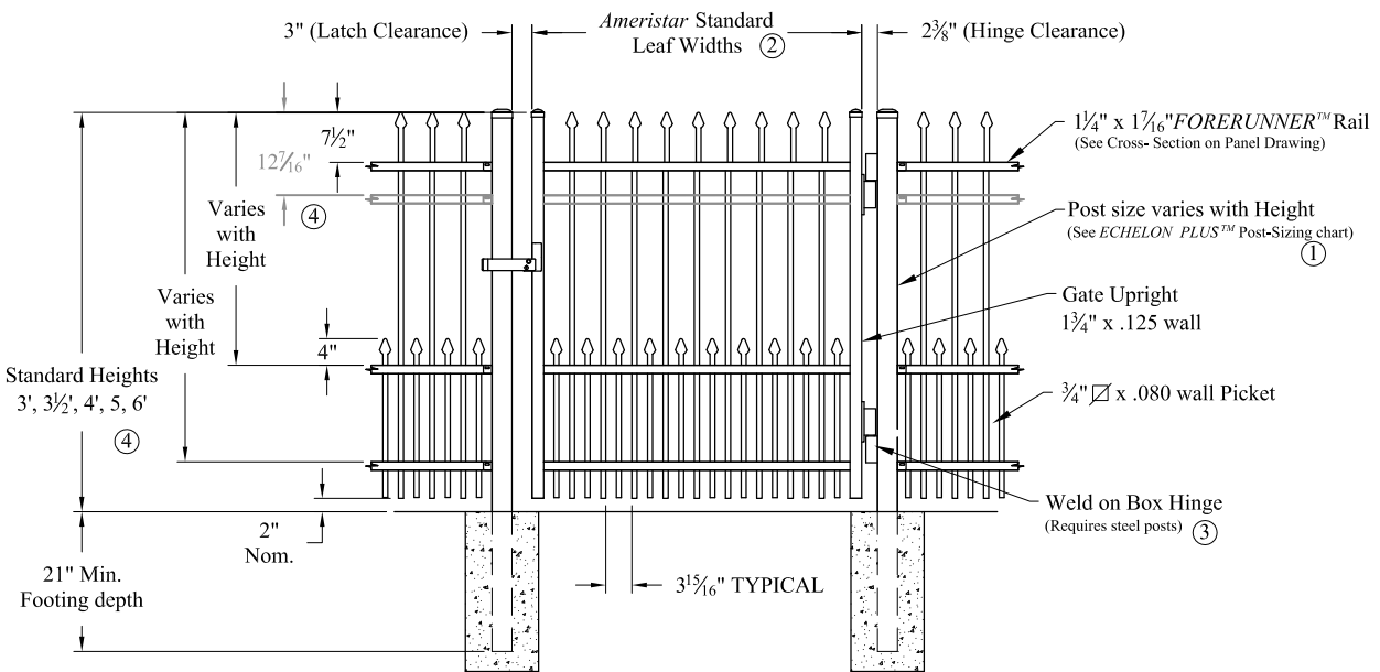
Single gate Arrangement
