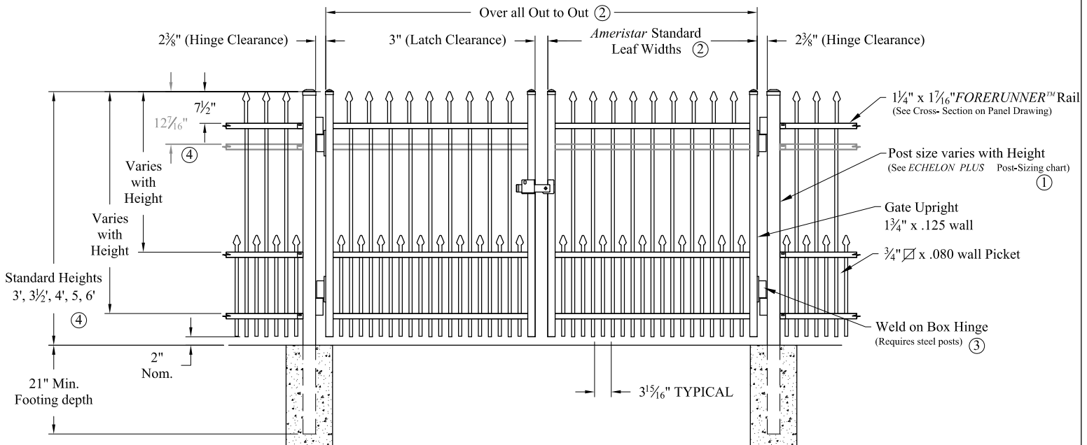
Double gate Arrangement
