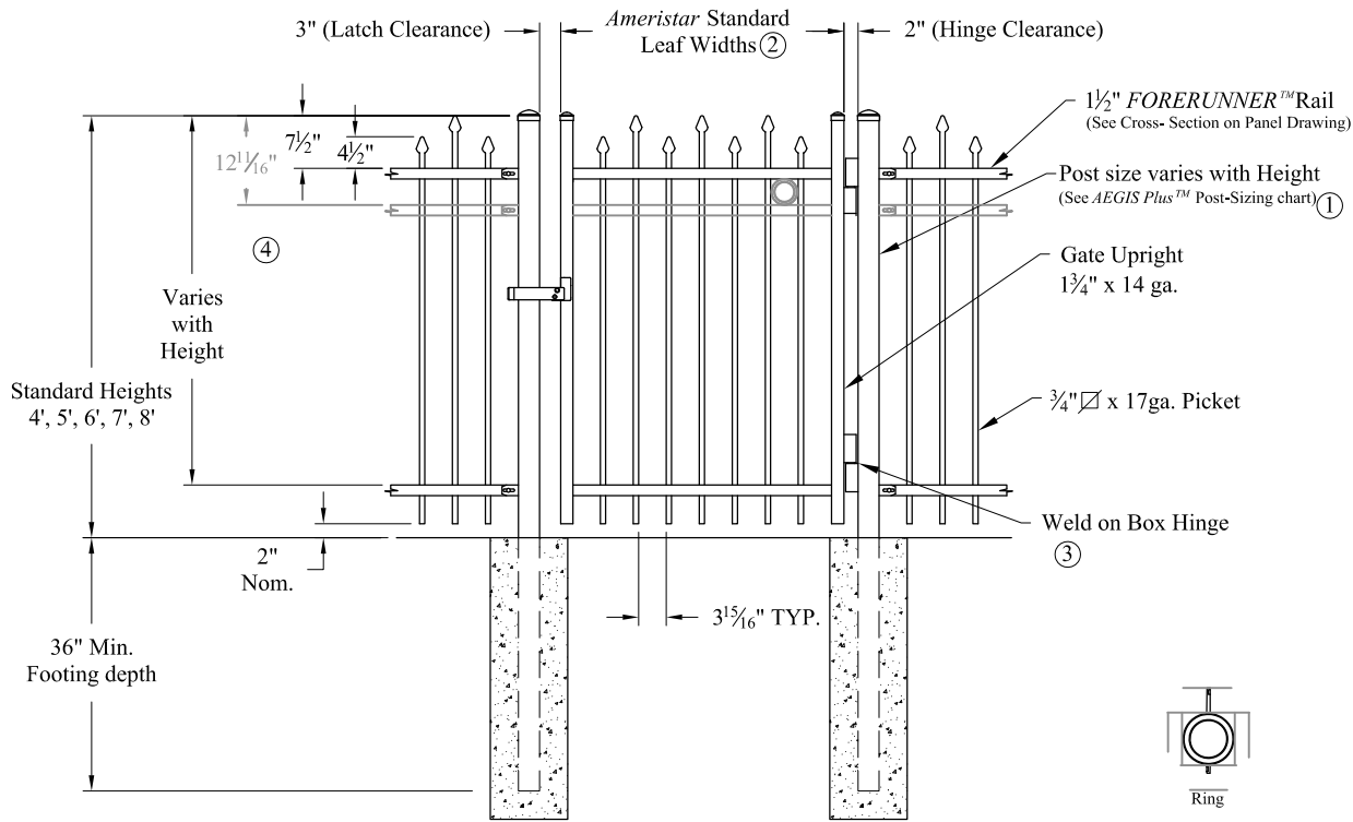
Single gate Arrangement
