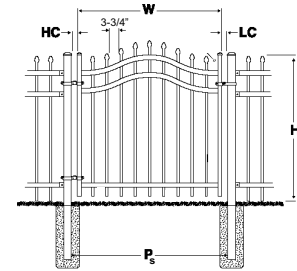
Order 1 Leaf For Single Swing Opening (Available only as single)
