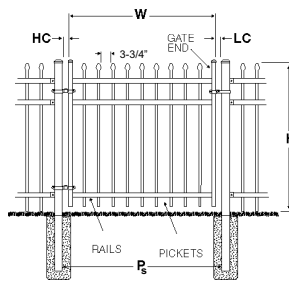
Order 1 Leaf For Single Swing Opening
